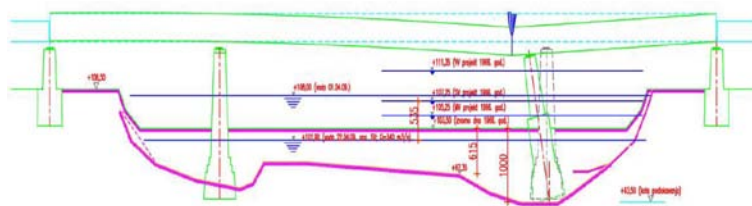
Figure 1 Influence of global and local erosion on the Sava river channel in the profile of the bridge "Jakuševac" during 20-year period.
