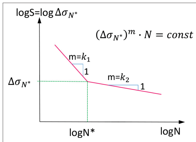
Figure 2 the corresponding S-N curve
