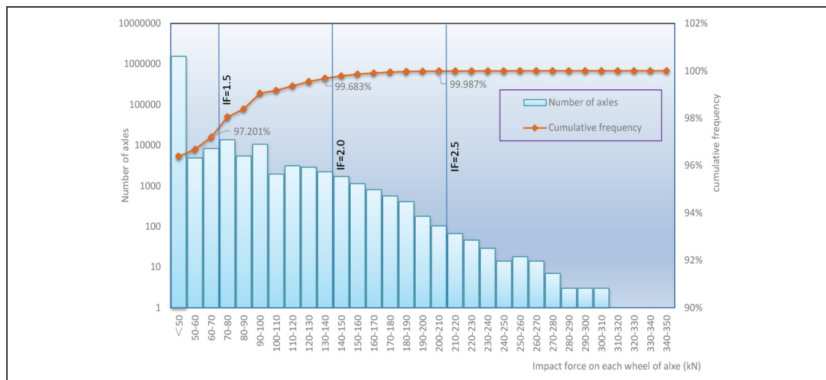
Figure 3 Typical impact force statistical data on track
