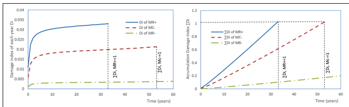
Figure 5 The damage index of each year and accumulated damage with time
