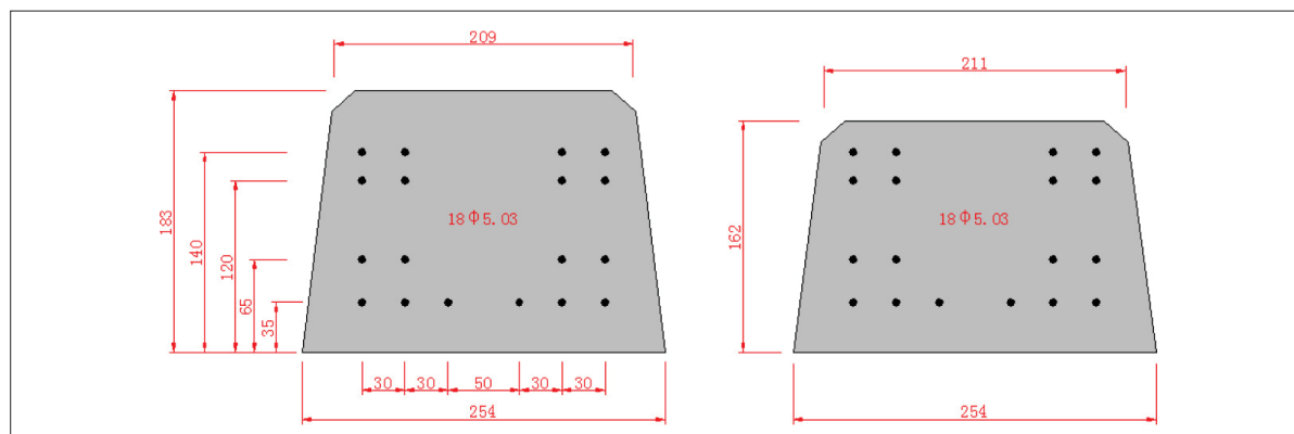
Figure 4 Railseat and centre section of sleeper
