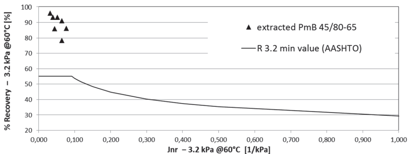
Figure 6 MSCRT results for PmB 45/80-65 extracted from asphalt mixes A to G.
