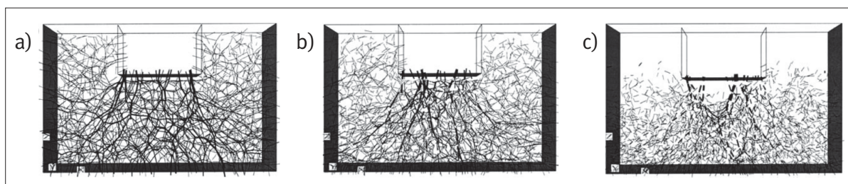
Figure 10 Contact forces after the compaction of the assembly for: a) spheres, b) clumps, c) clumps with smaller diameter, [24]
